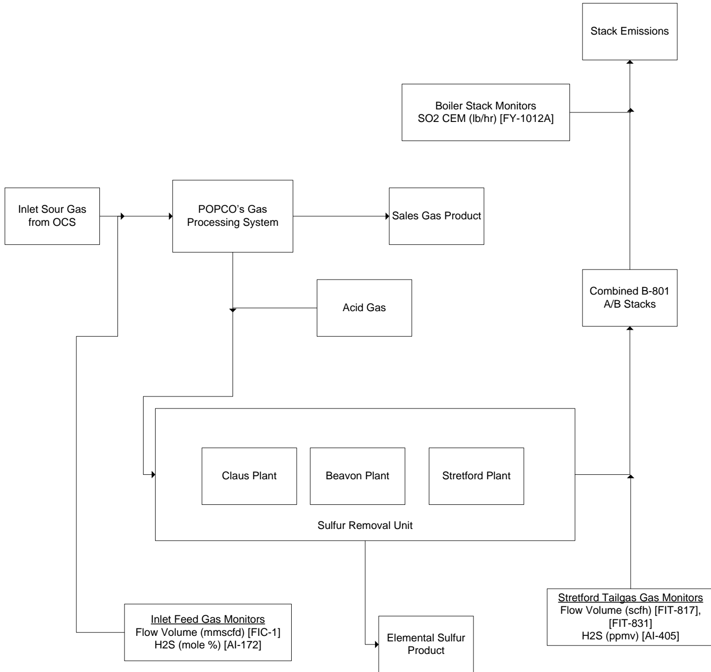
Figure 3.1 POPCO SRU BACT & NSPS Monitoring Systems
