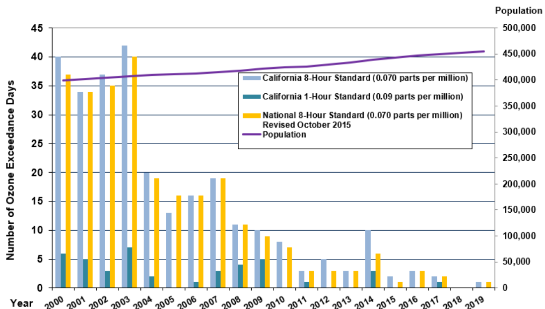
Santa Barbara County Ozone Exceedance Days 2000-2019
