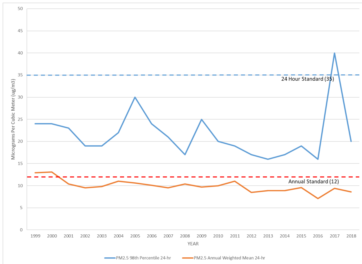
FIGURE 5-9: MEASURED PM 2.5 LEVELS (µg/m 3 )
