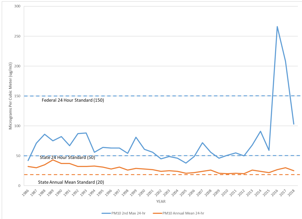
FIGURE 5-8: MEASURED PM 10 LEVELS ( \mu\text{g}/\text{m}^3 ) 1
